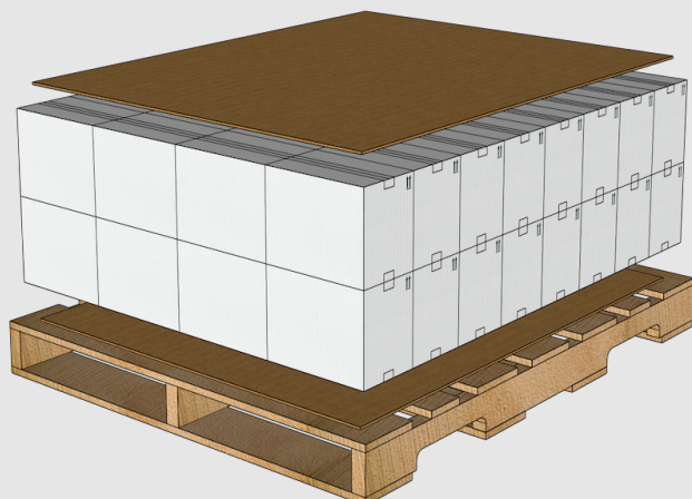
Full Pallet Dimensions - 48" x 42" x 21"
