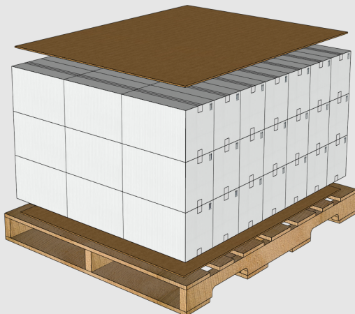
Full Pallet Dimensions - 48" x 40" x 23"
