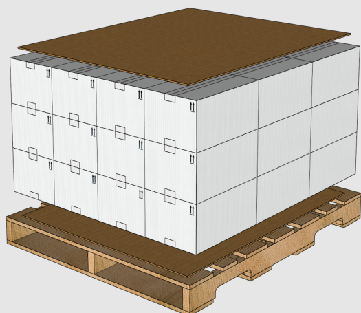
Full Pallet Dimensions - 48" x 40" x 30"
