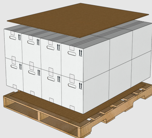
Full Pallet Dimensions - 48" x 40" x 36"
