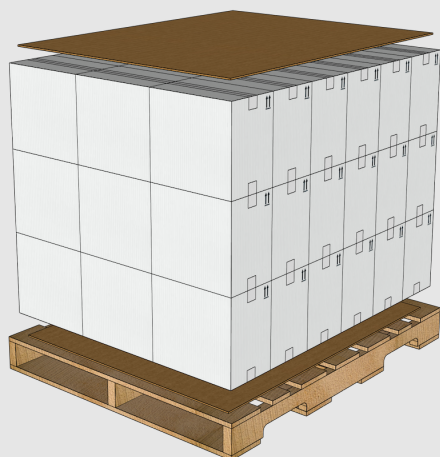
Full Pallet Dimensions - 48" x 44" x 32"
